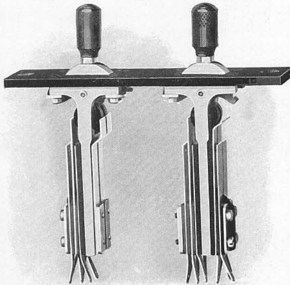
Fig. No. 8632—Code Nos. 1041 and 1033 Keys on No. 1013 Escutcheon
