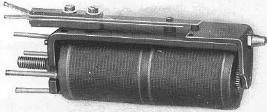
Fig. No. 8616—Code No. 2030 Cord Circuit Relay
