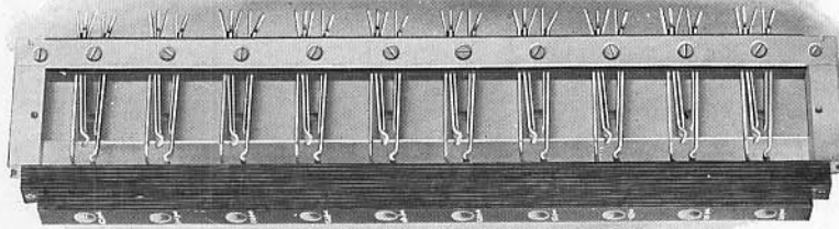
Fig. No. 8630—Code No. 267 Spring Jack
