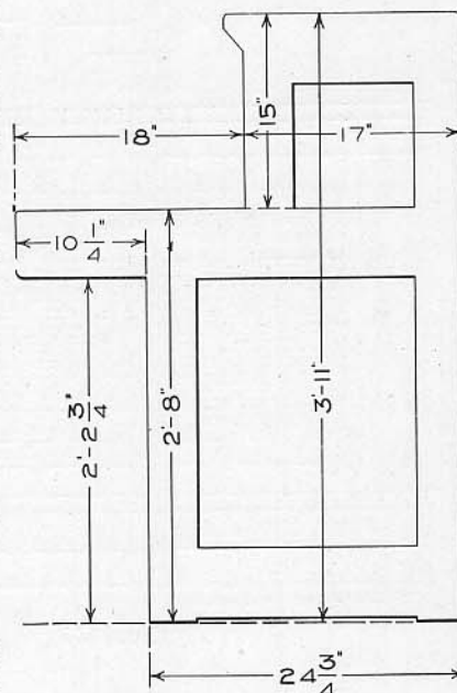
Fig. No. 8612 Side Elevation Code No. 101 Cabinet
